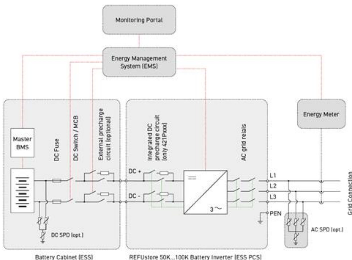
Figure 5 – Scheme of an installation
