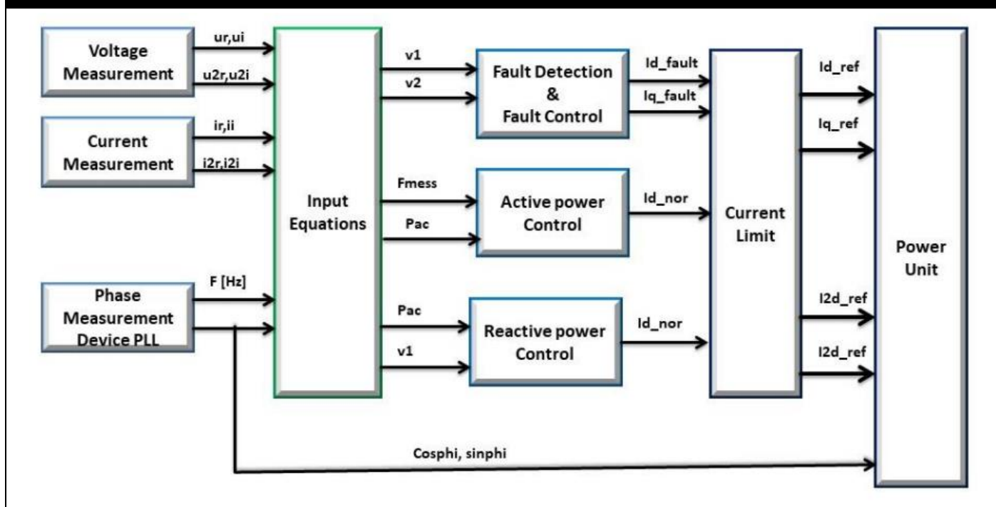
Figure 20 – Control frame of the simulation model
