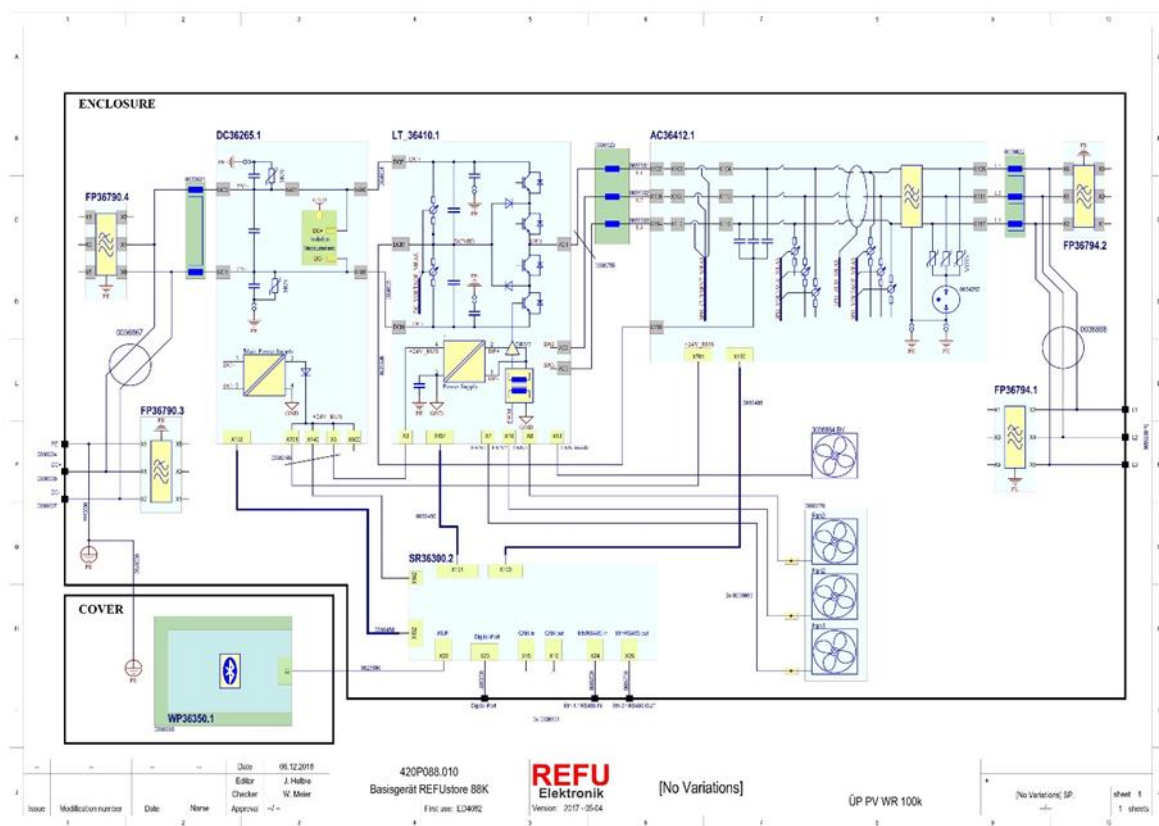
Figure 3 – Block diagram of the battery inverter
