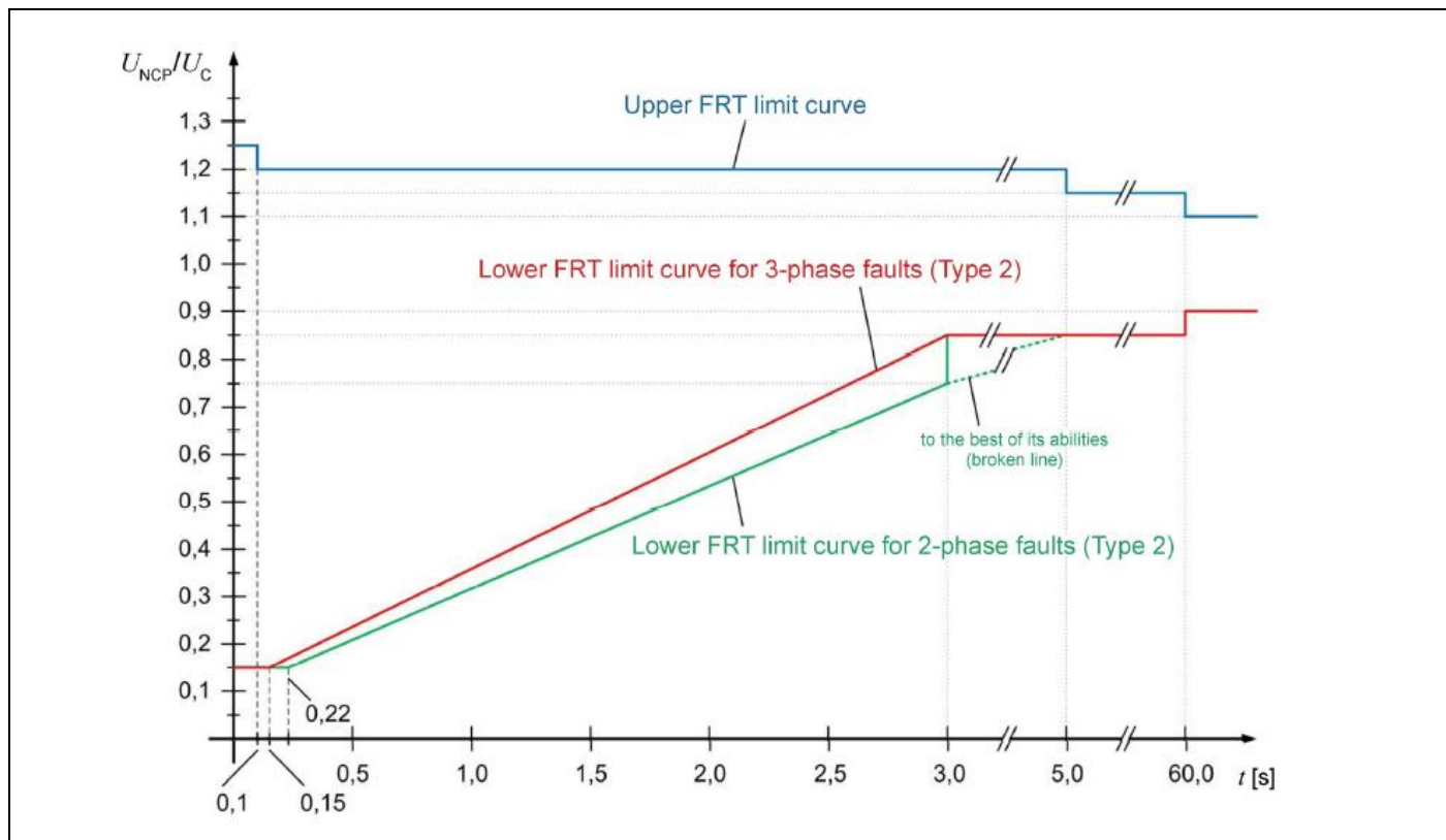
Figure 15 – Verified Fault Ride-Through (FRT) limit curve from [6]
