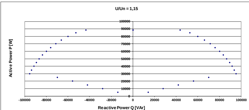
Figure 13 – Voltage dependent PQ operating points from [15]
